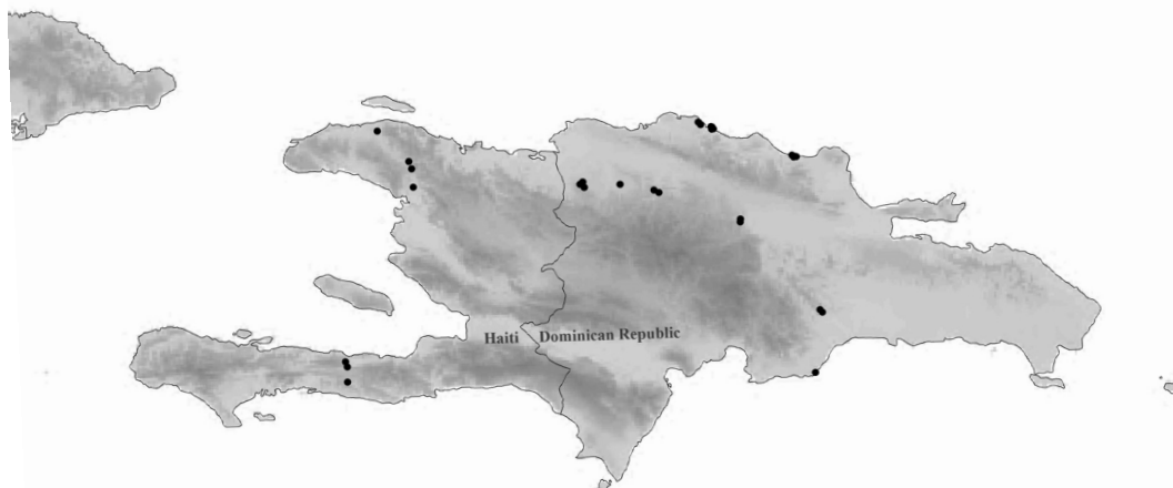
6. Distribution of Zombia antillarum in Hispaniola.
